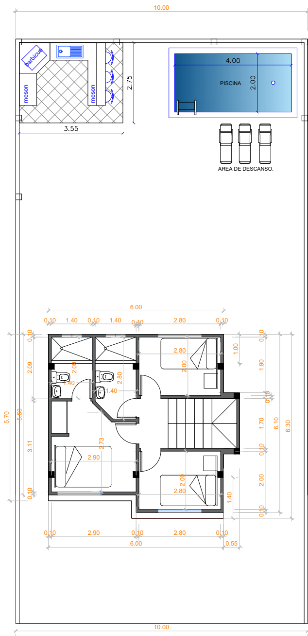
VILLA OCEANICA 2 PLANTA ALTA N+3.18
